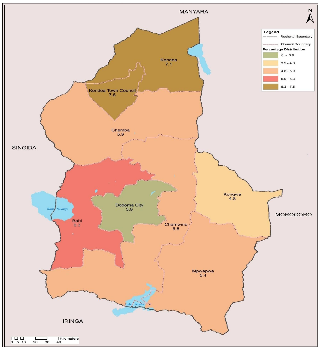
Map 3. 30: Percentage Distribution of Projected Population Aged 65 Years and Above by Council; Dodoma Region, 2050
